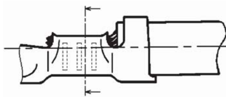
Figure 32 – Microsection plane
