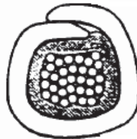
Figure 26 – Cross section of insulation crimp, type C
