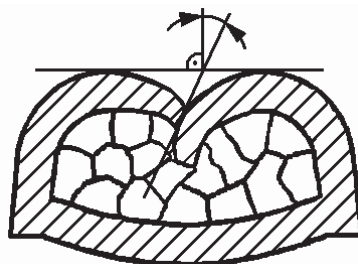
Figure 12 – Supporting angle
