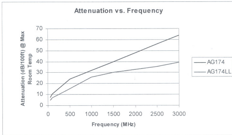
FIGURE 3: Maximum Attenuation Values
