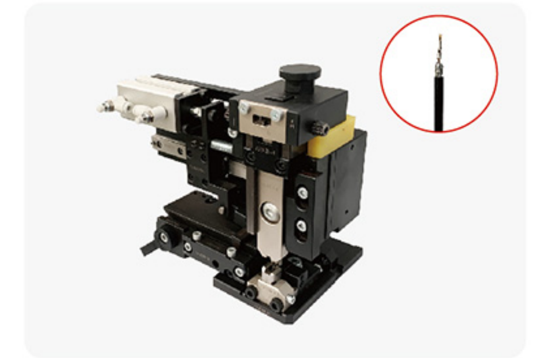
YIM-AFS300M Crimping Applicator
