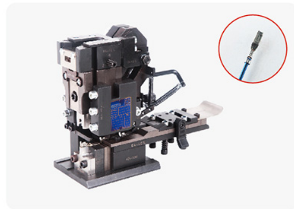
E4 Crimping Applicator
