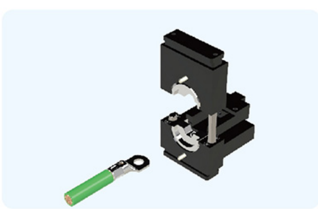
WHCA Crimping Applicator
