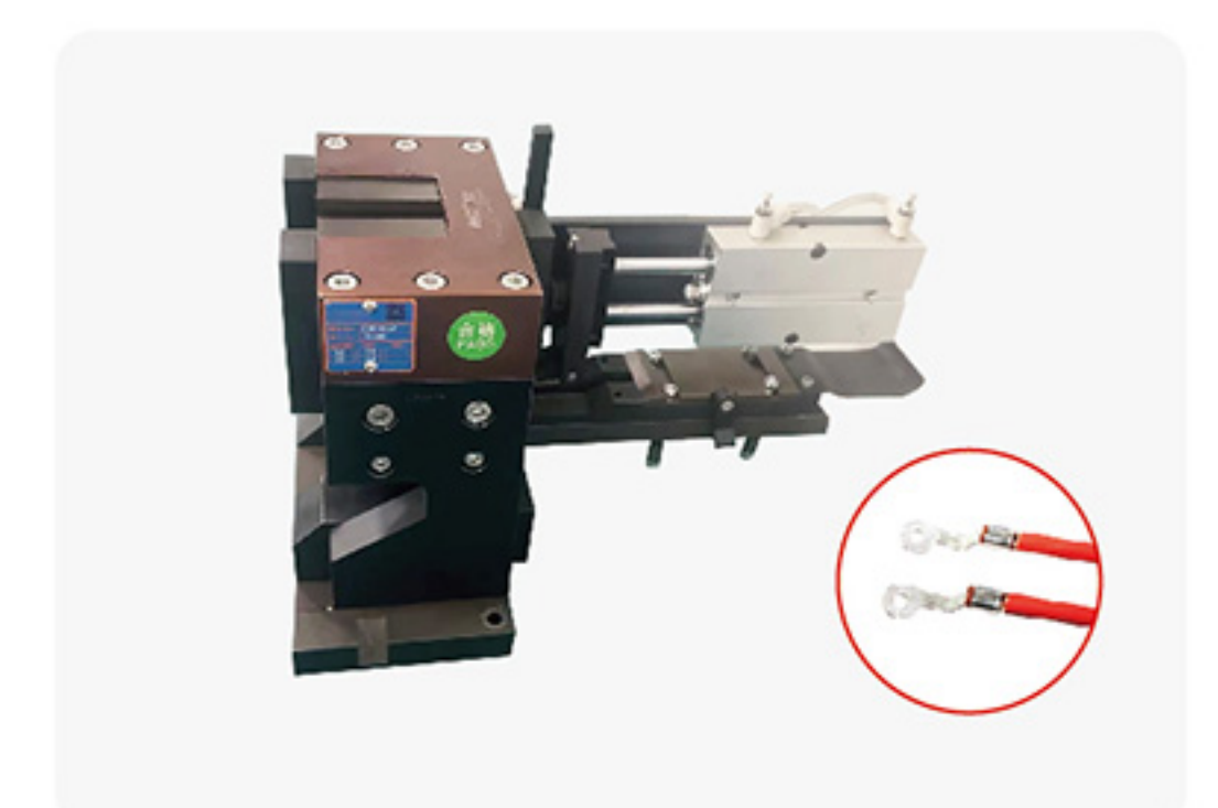
LCME Crimping Applicator
