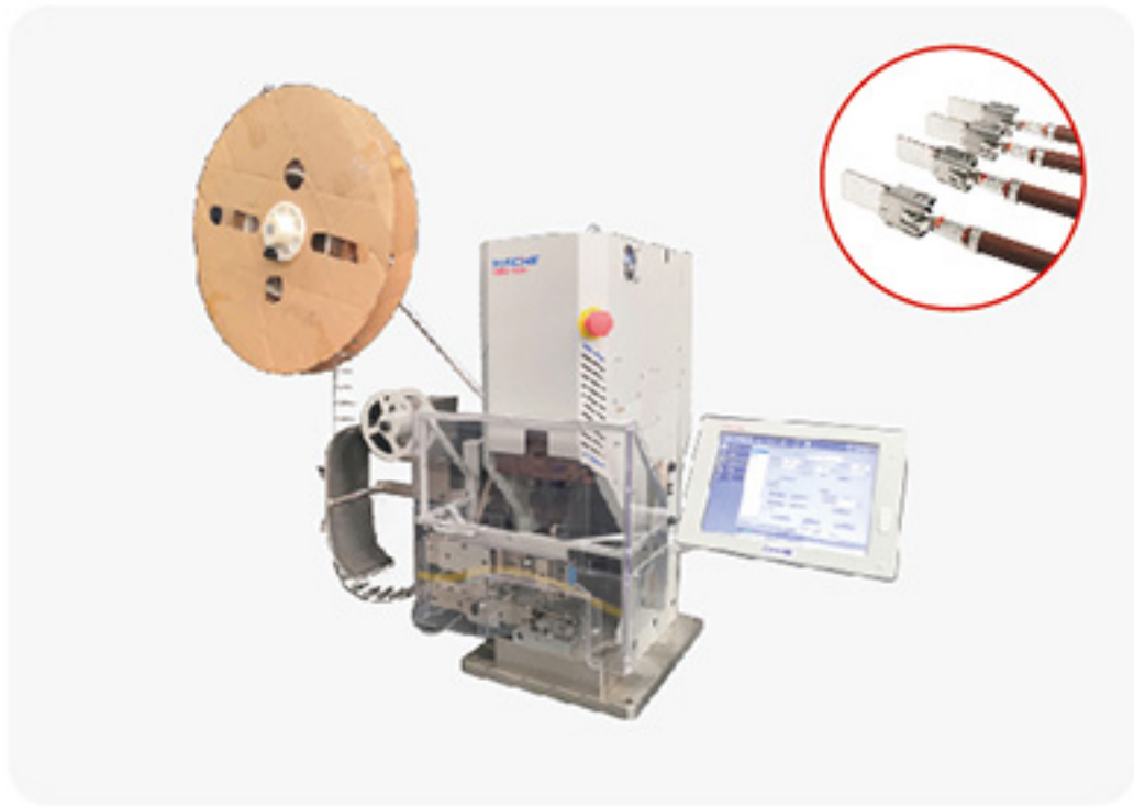
HBQ - 160H Multi - Functional Servo Crimping Machine
