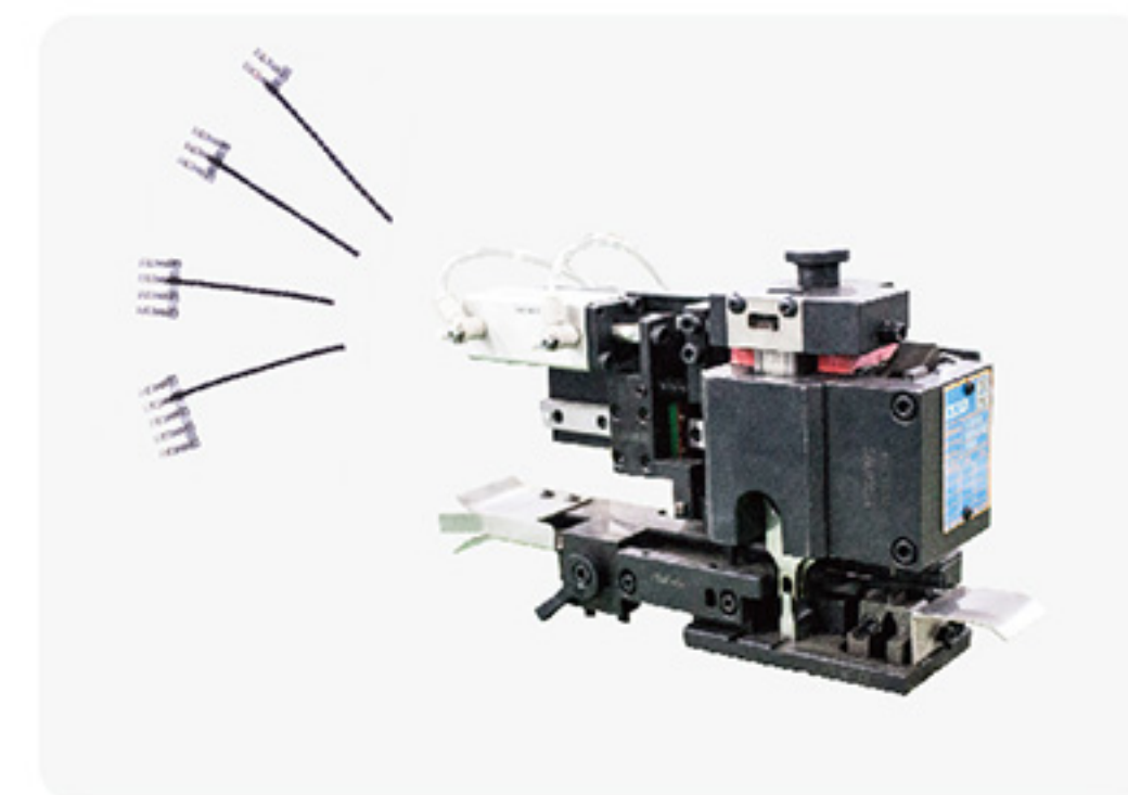
AFTCA Counting Crimping Applicator
