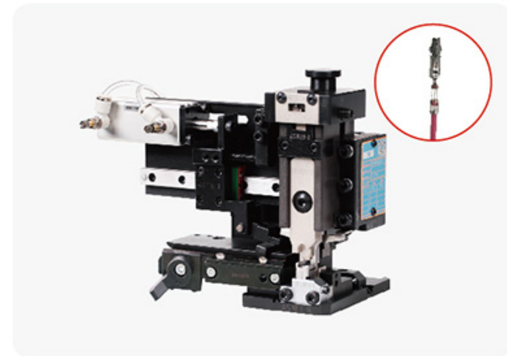
YJM-AFS300I Crimping Applicator
