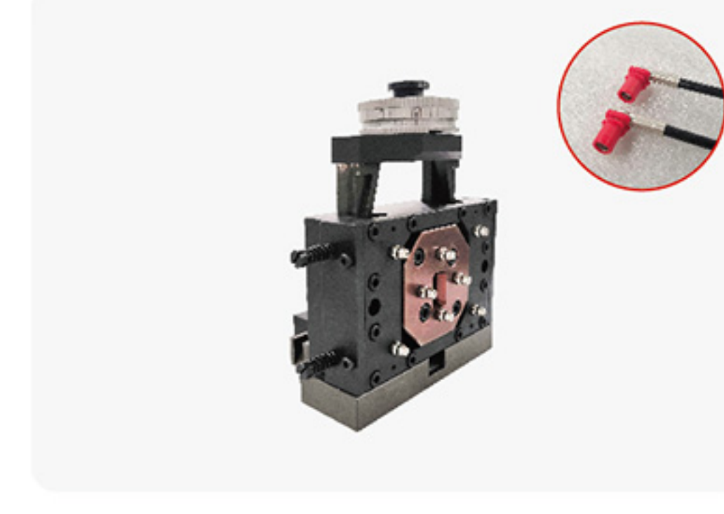
RFPCA Crimping Applicator
