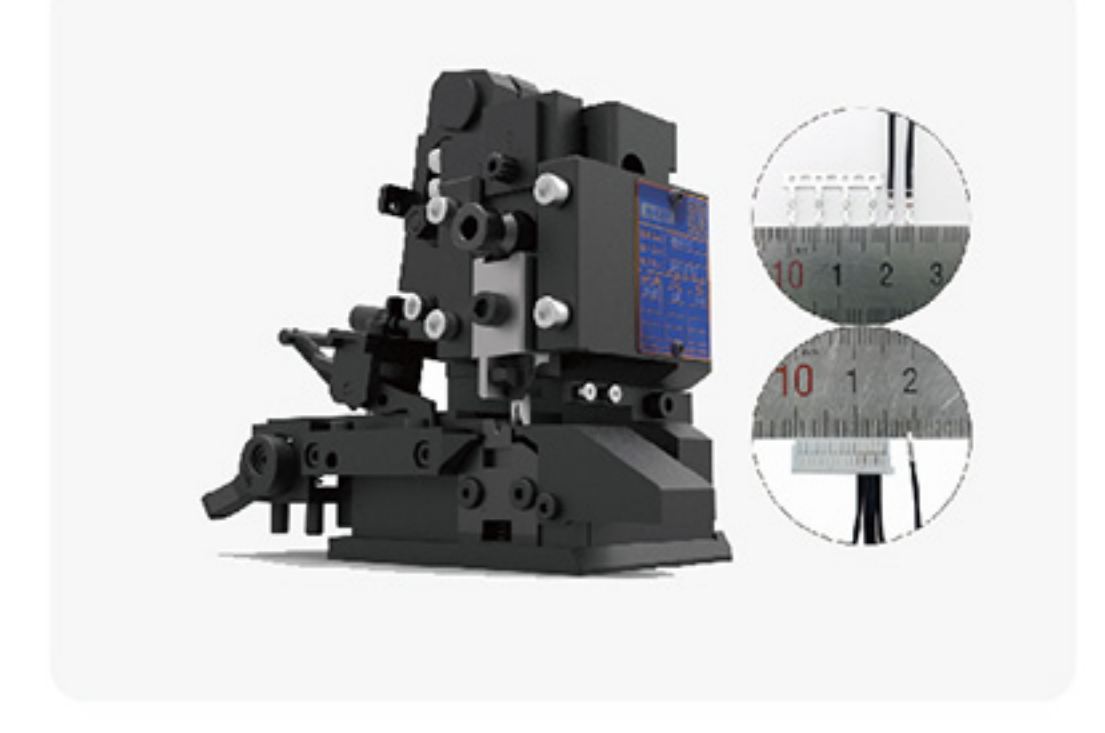
NANO Crimping Applicator (S4B)
