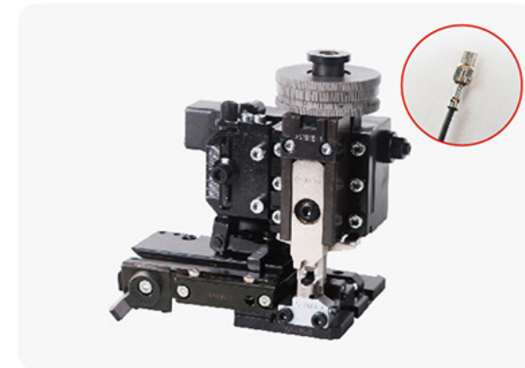
S3D Crimping Applicator
